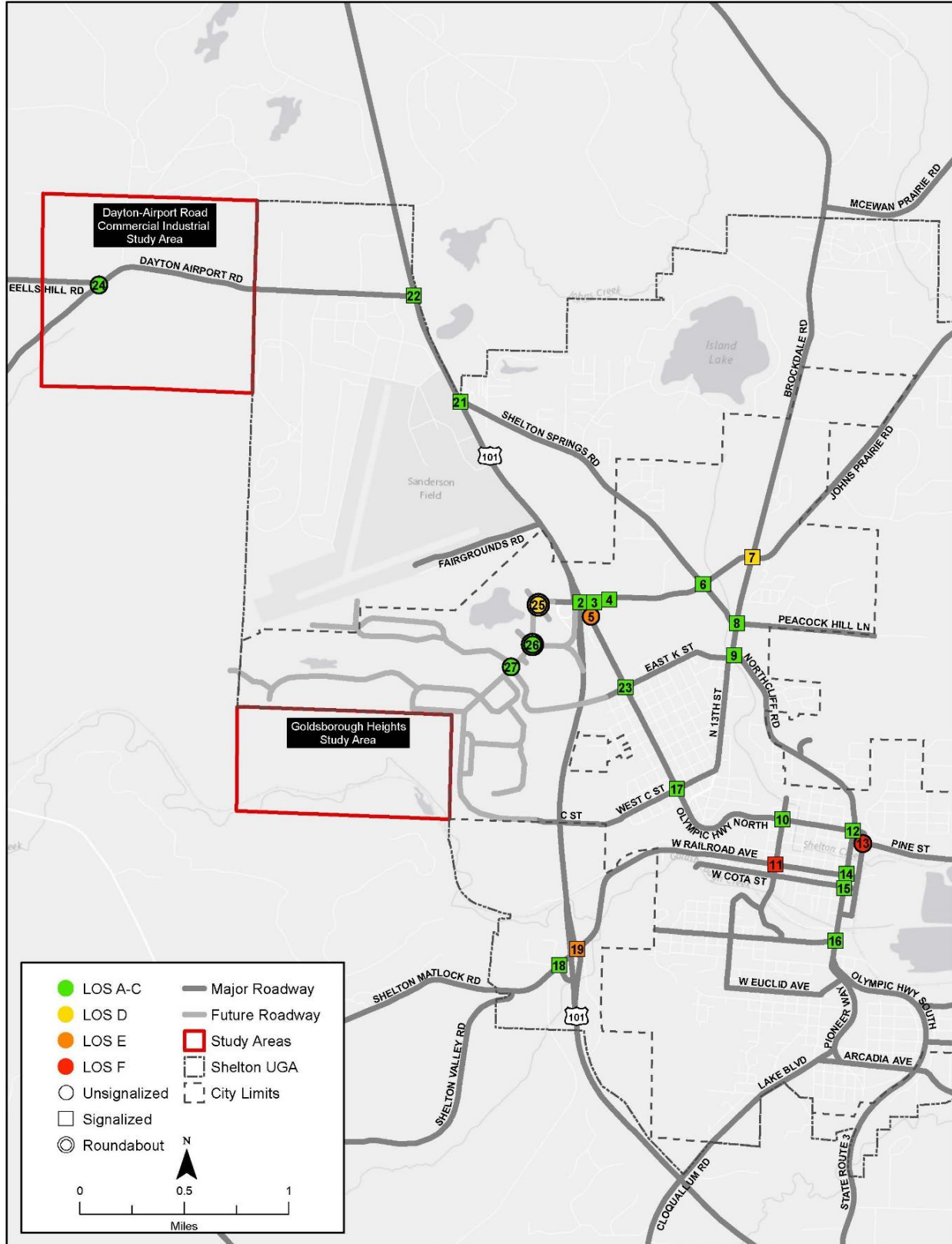
Figure 15 – 2036 Intersection Operations
